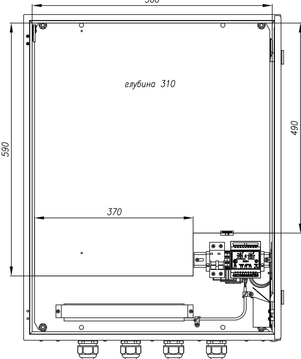
ТШ-2 (600x760x350) 560
