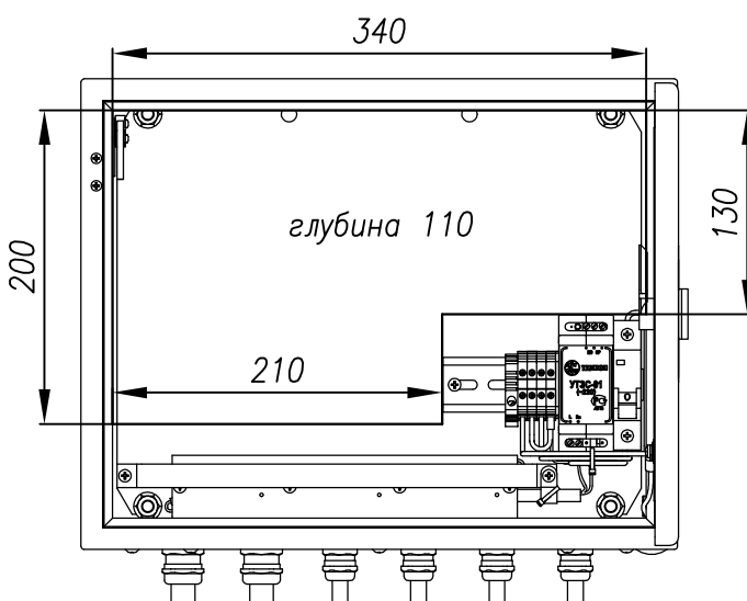
ТШ-6 (300x380x155) 340
